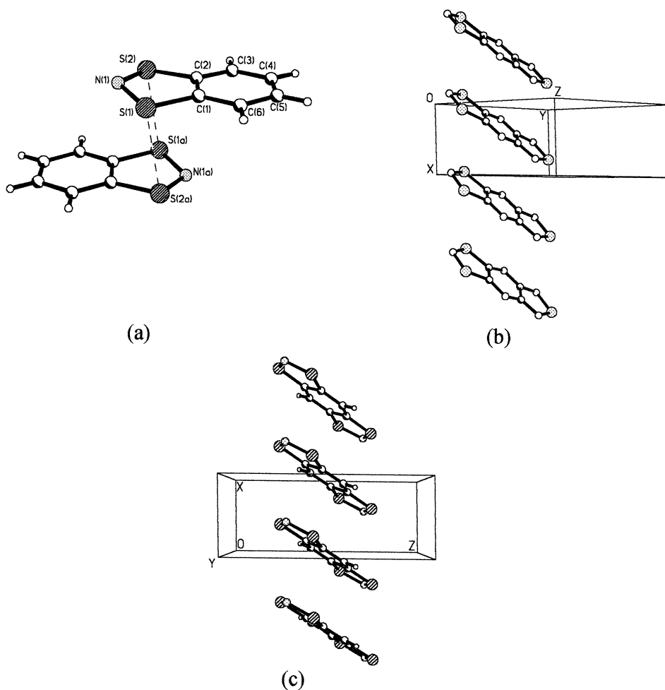
Fig. 4. Solid state structures of (a) dimeric 34• , (b) monomeric 27• and (c) the diradical 28•• .
